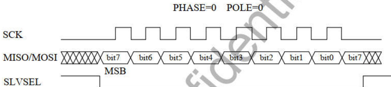
Figure 2-9 SPI Data Transfer Format (Phase=0, POLCK=0)
