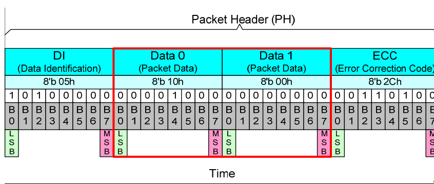
Figure 54 Packet Data (PD) for Short Packet (SPa), 1 Byte Information
