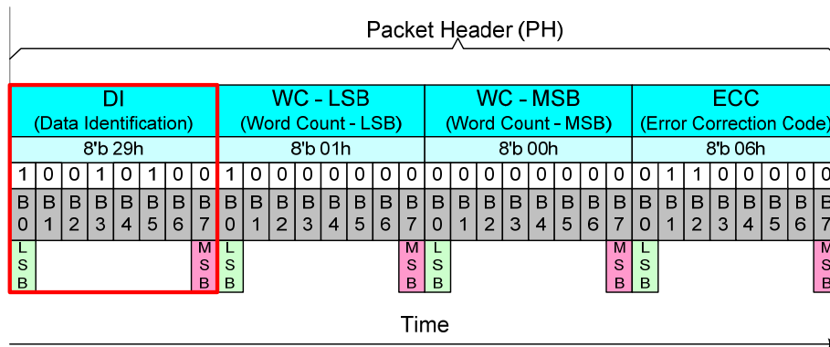
Figure 49 Data Identification (DI) on the Packet Header (PH)
