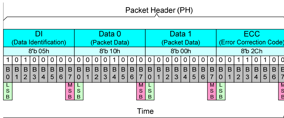
Figure 68 Display Command Set (DCS) Write, No Parameter (DCSWN-S) - Example
