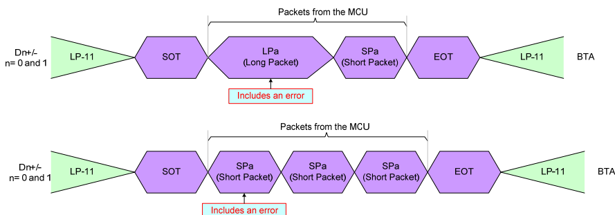
Figure 82 Errors Packets
