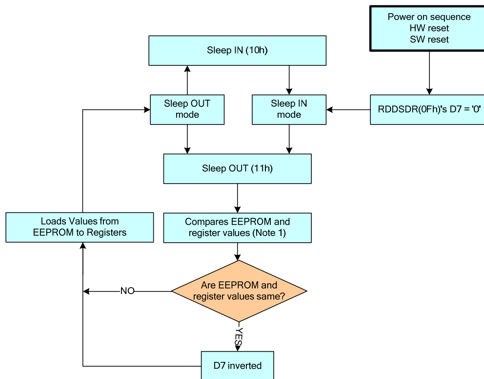
Figure 98 Register loading Detection
