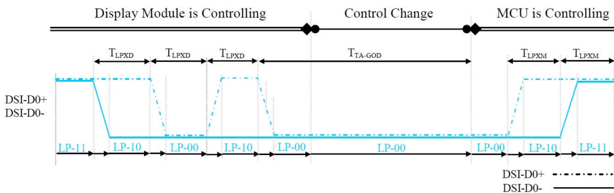
Figure 119 BTA from the Display Module to the MPU
