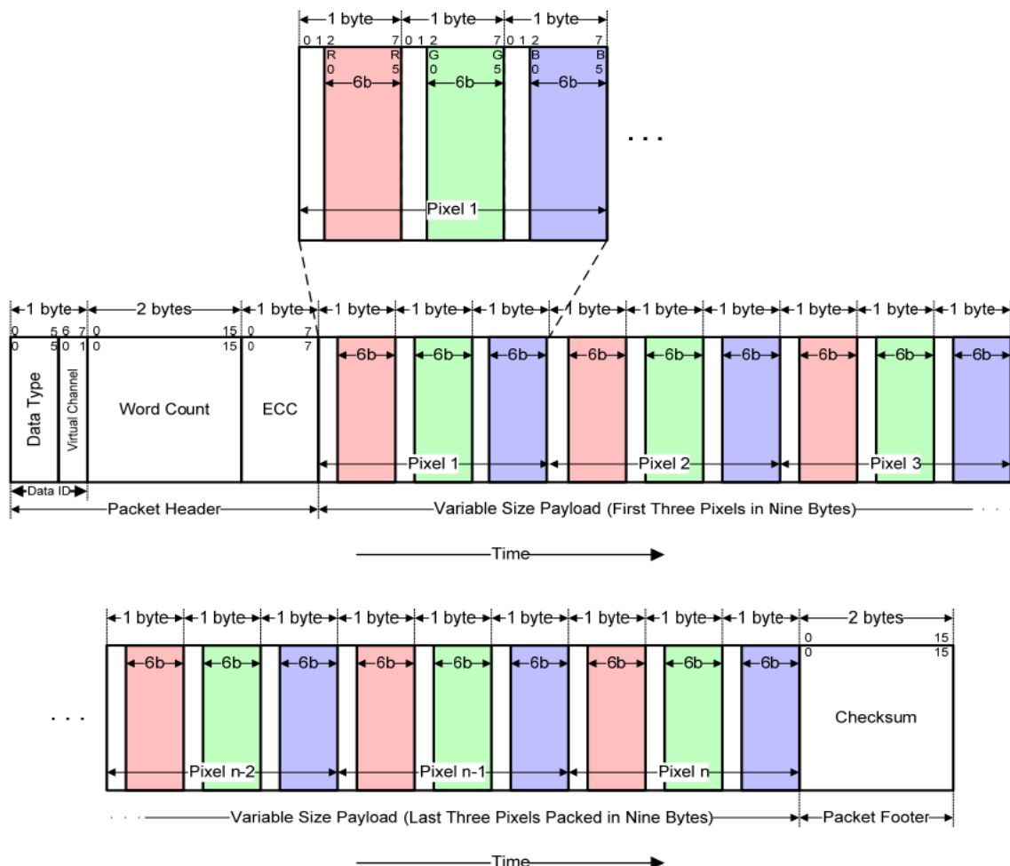
Figure 92 18-bit per Pixel, Data Type = 10 1110 (2Eh)
