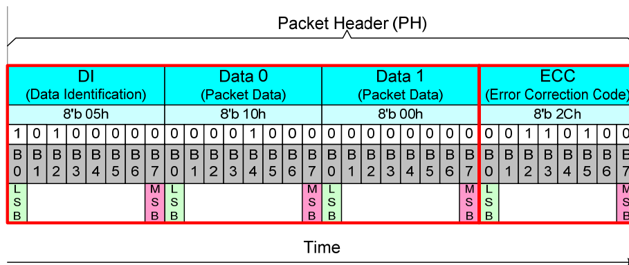
Figure 57 D[23...0] and P[7...0] on the Short Packet (SPa)
