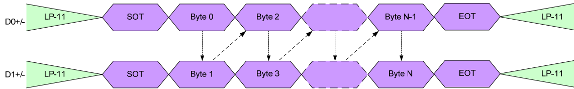
Figure 34 Single Packet in HSDT – Even Number of Bytes
