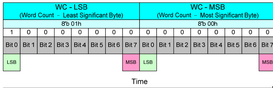
Figure 45 Byte Order of the Multiple Byte Information on Packets
