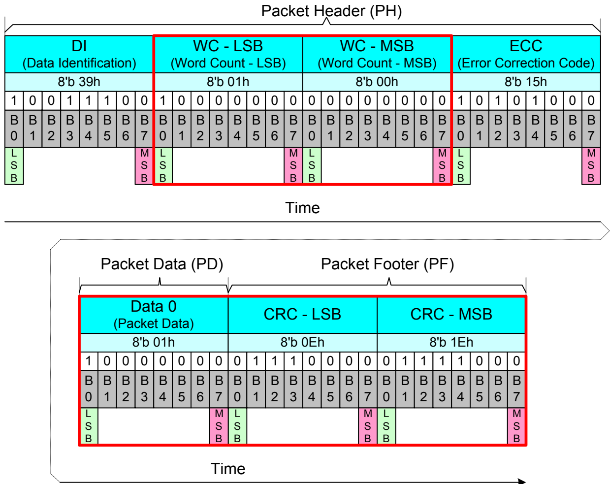
Figure 66 Packet Footer (PF) Example
