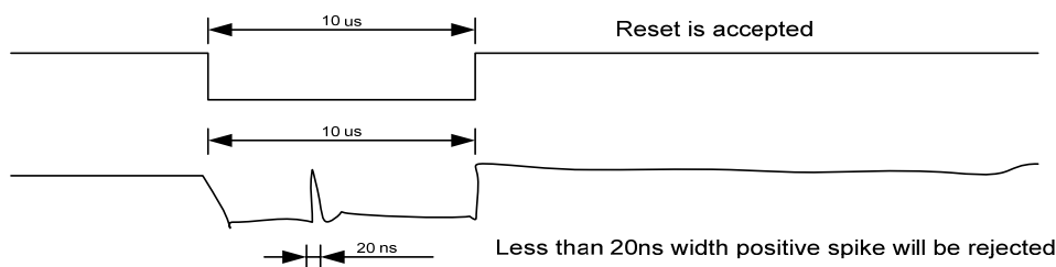
Figure 104 Positive Noise Pulse during Reset Low
