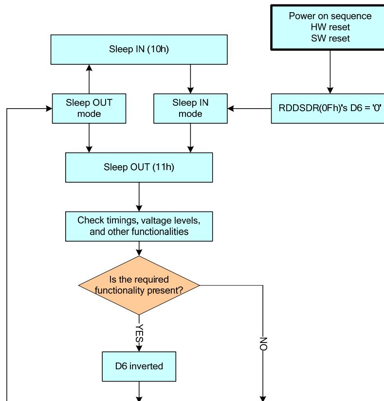
Figure 99 Functionality Detection
