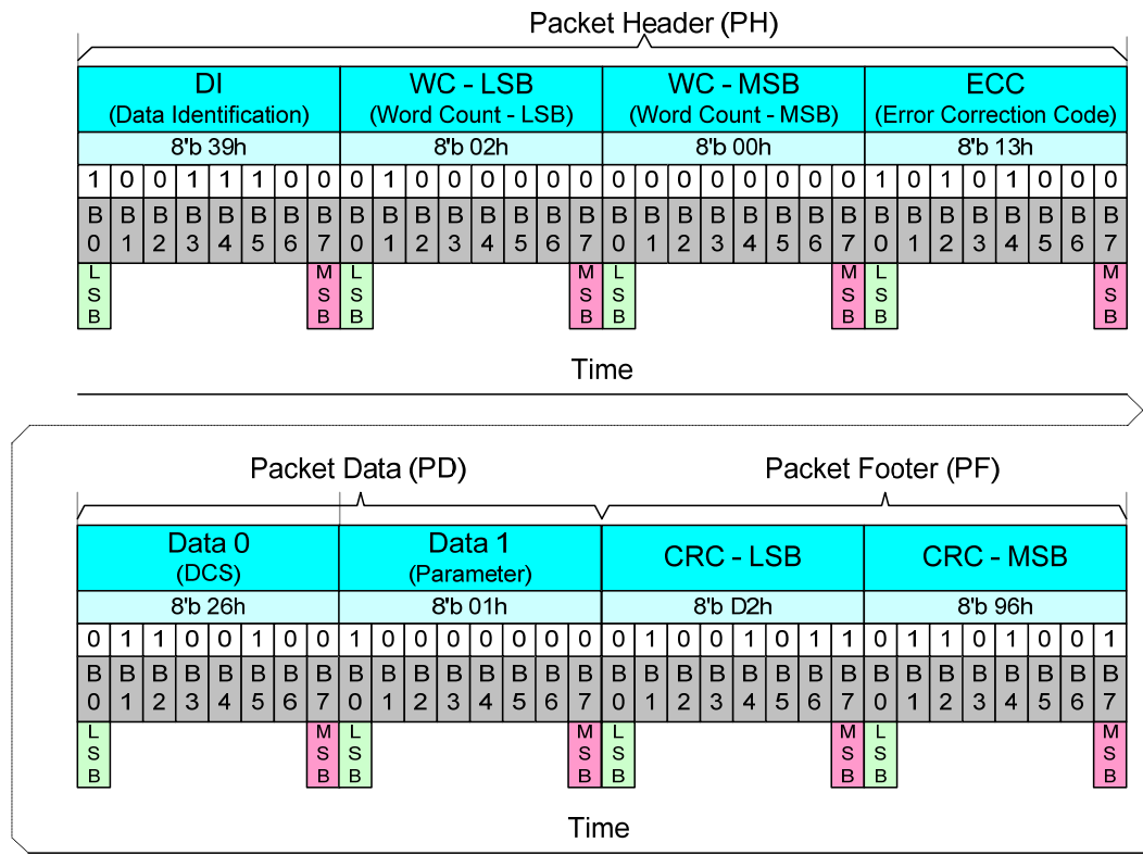
Figure 71 Display Command Set (DCS) Write Long with DCS and 1 Parameter - Example
