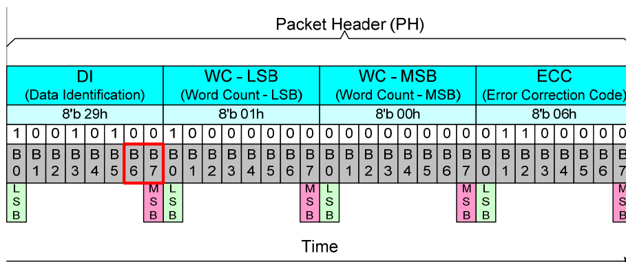
Figure 50 Virtual Channel (VC) on the Packet Header (PH)
