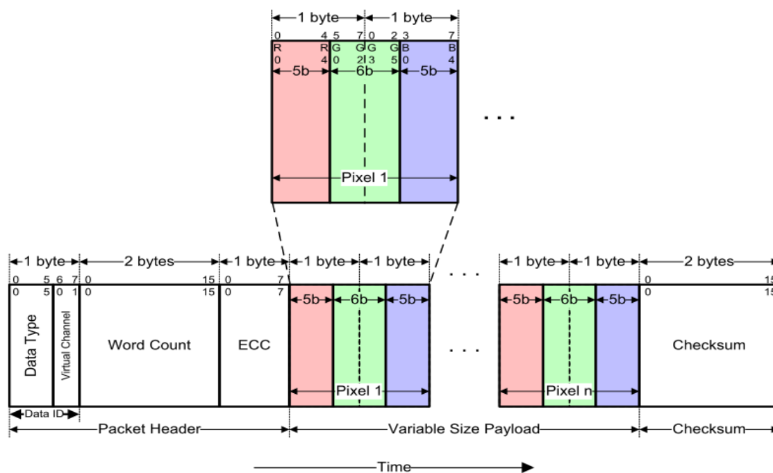
Figure 90 16-bit per Pixel, Data Type 00 1110 (0Eh)
