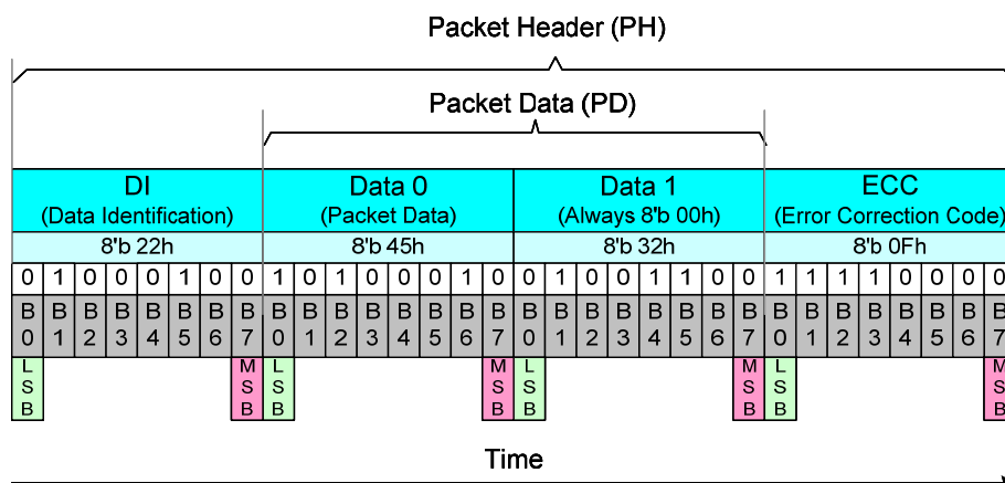
Figure 86 DCS Read Short Response, 2 Bytes Returned (DCSRR2-S) - Example
