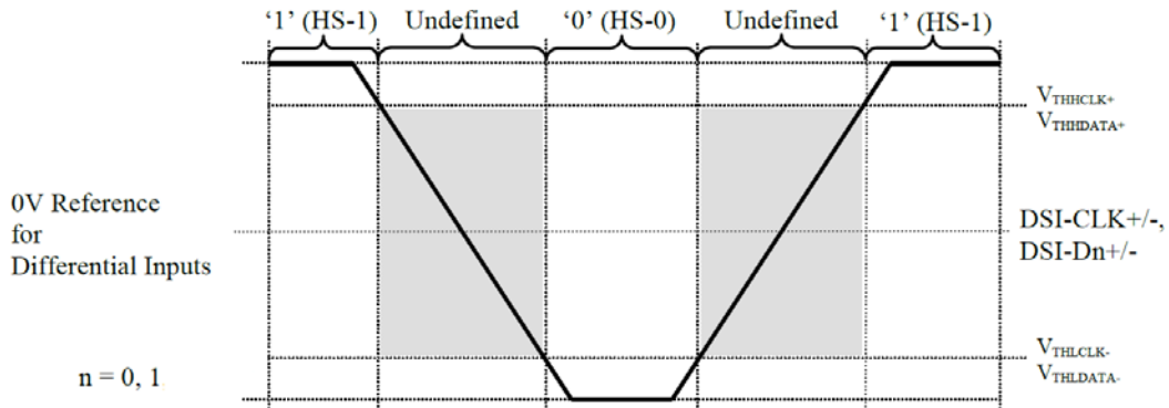
Figure 112 Differential Inputs Logical '0's and '1's, Threshold High/Low, Differential Voltage Range
