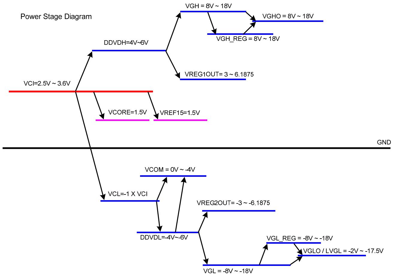
Figure 101 Power Stage Diagram
