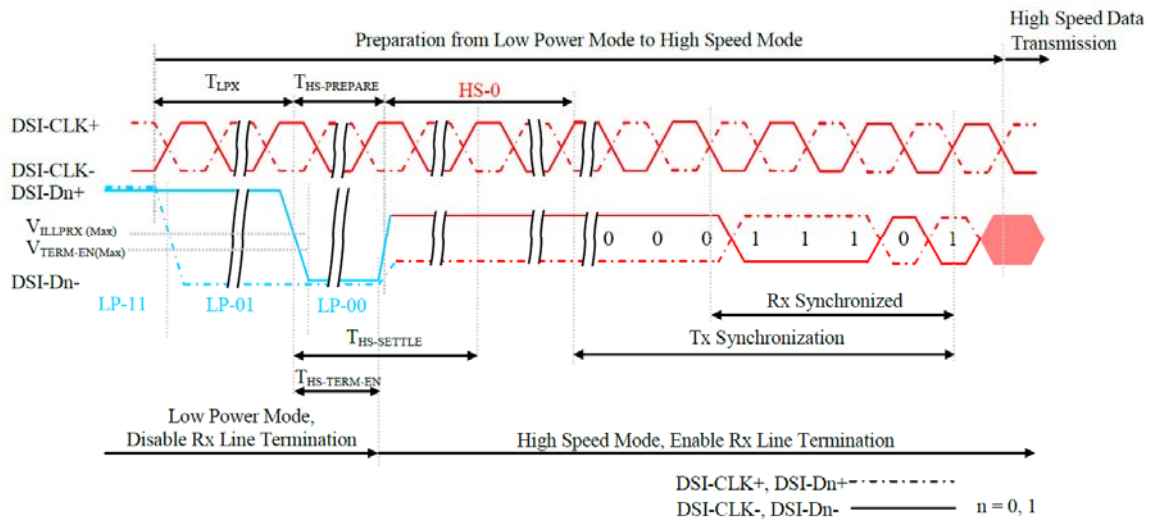
Figure 120 Data Lanes – Low Power Mode to High Speed Mode Timings
