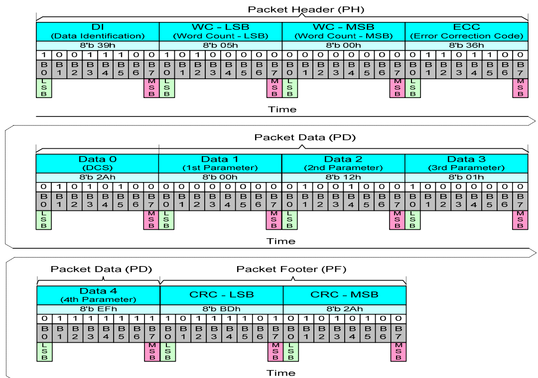
Figure 72 Display Command Set (DCS) Write Long with DCS and 4 Parameters - Example
