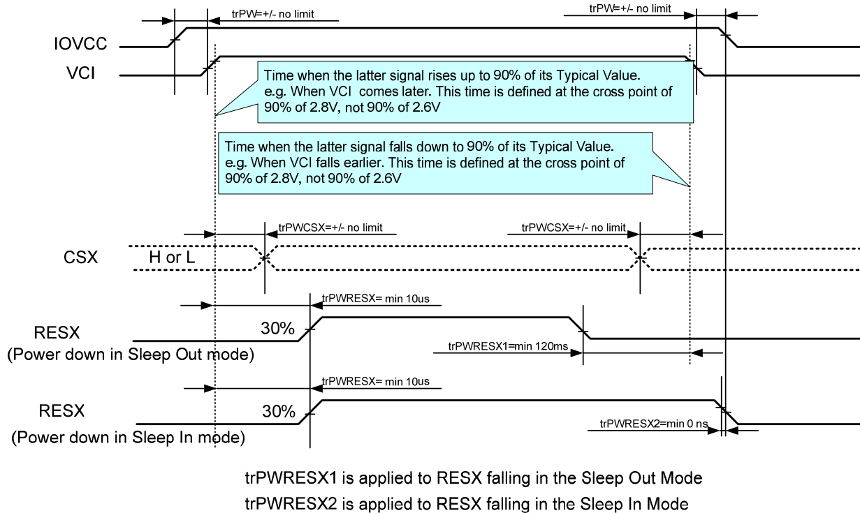
Figure 100 Case 2 – RESX line is held Low by Host at Power ON
