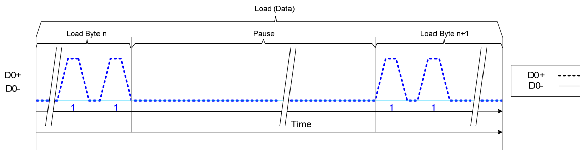
Figure 25 Pause (Example)
