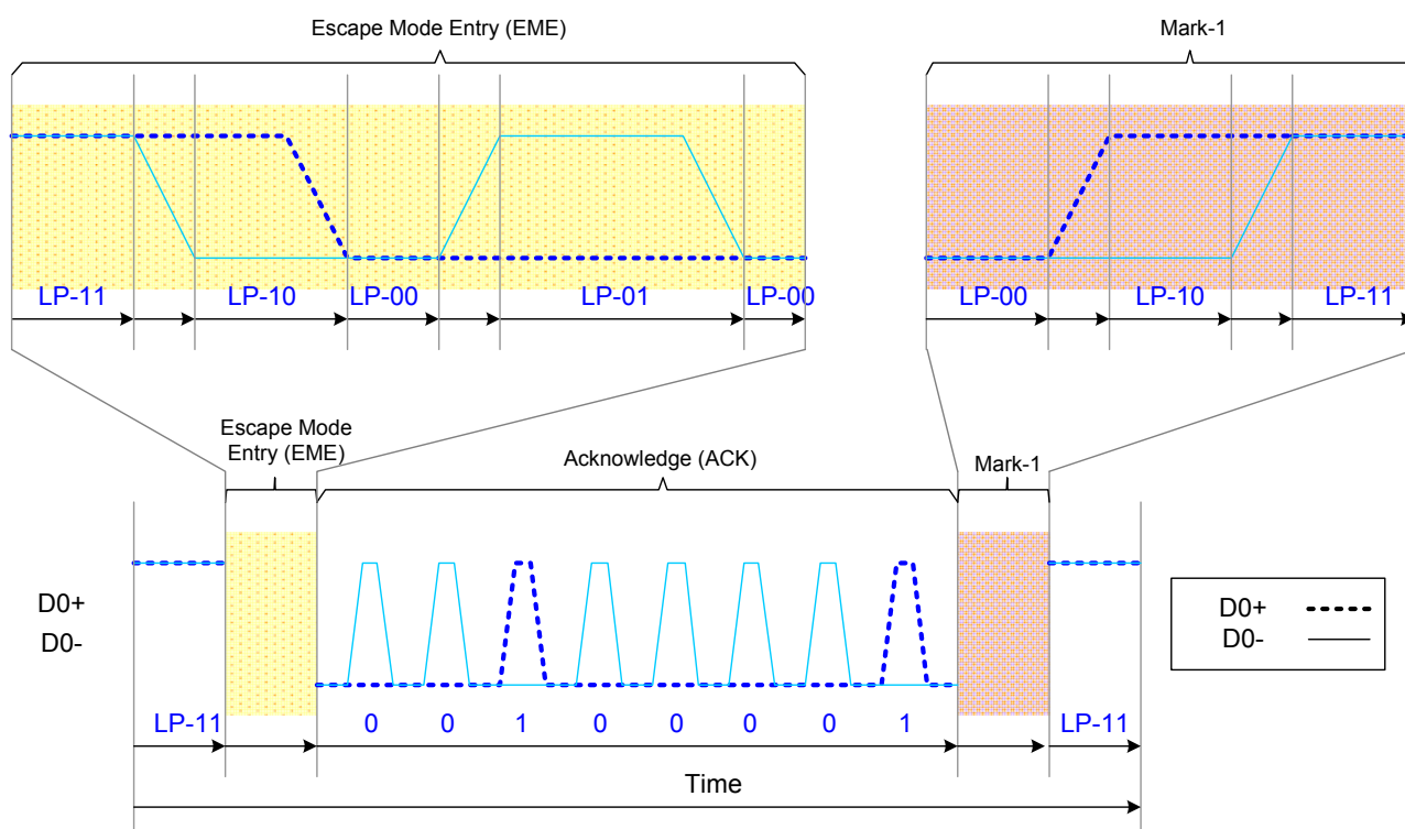
Figure 28 Acknowledge (ACK)
