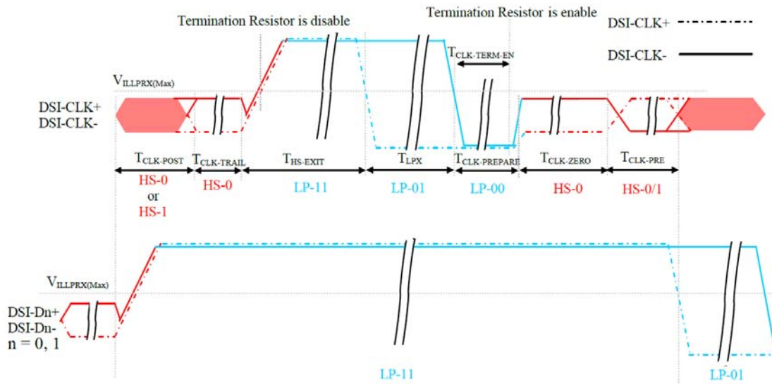
Figure 122 Clock Lanes – High Speed Mode to/from Low Power Mode Timings
