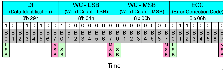
Figure 44 Bit Order of the Byte on Packets
