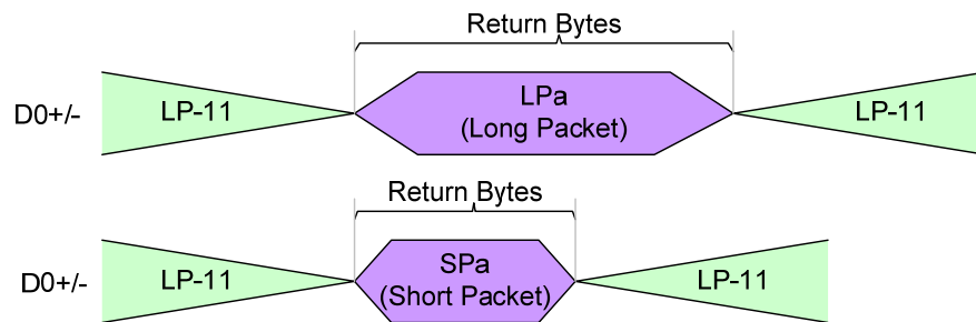
Figure 78 Return Bytes on Single Packet
