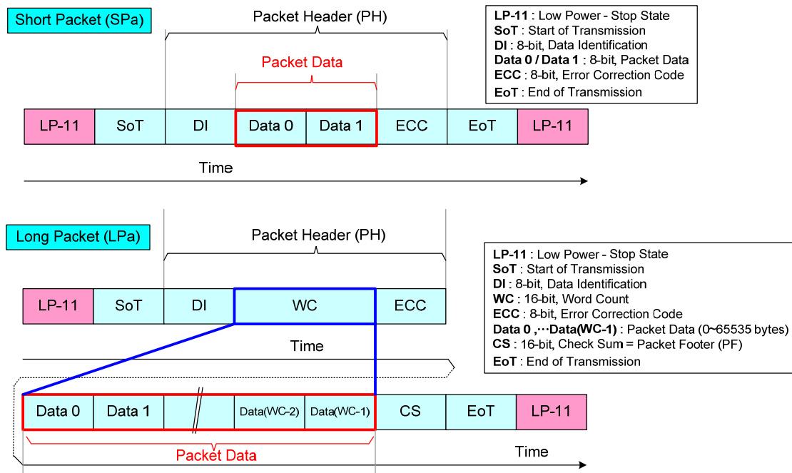
Figure 56 Packet Data in Short and Long Packets
