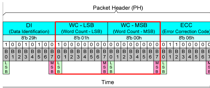
Figure 55 Word Count (WC) on the Long Packet (LPa)
