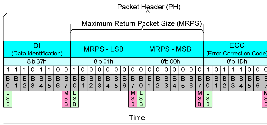
Figure 73 Set Maximum Return Packet Size (SMRPS-S) - Example
