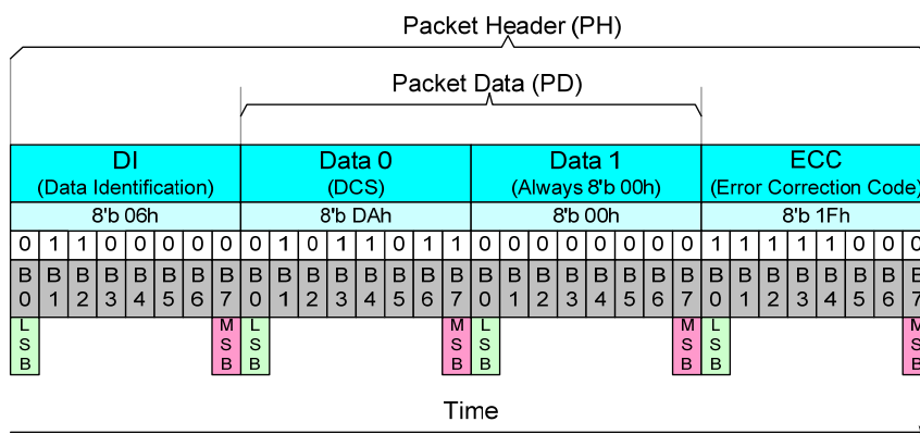
Figure 74 Display Command Set (DCS) Read, No Parameter (DCSRN-S) - Example
