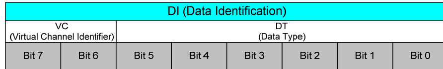
Figure 48 Data Identification (DI) Structure
