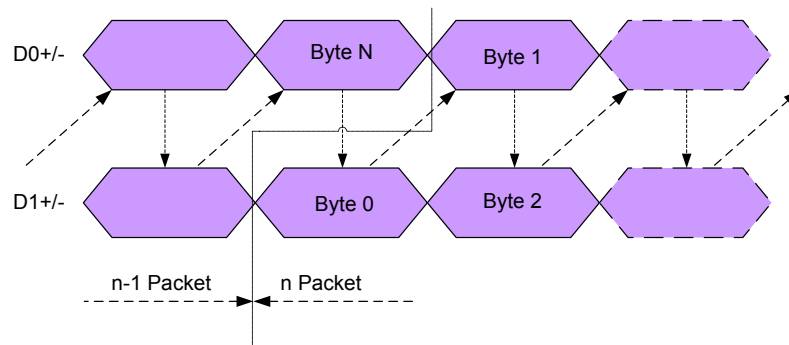
Figure 38 Continue Multiple Packets in HSDT when Number of Bytes is not Equal on Both Data Lanes at the End of the Packet
