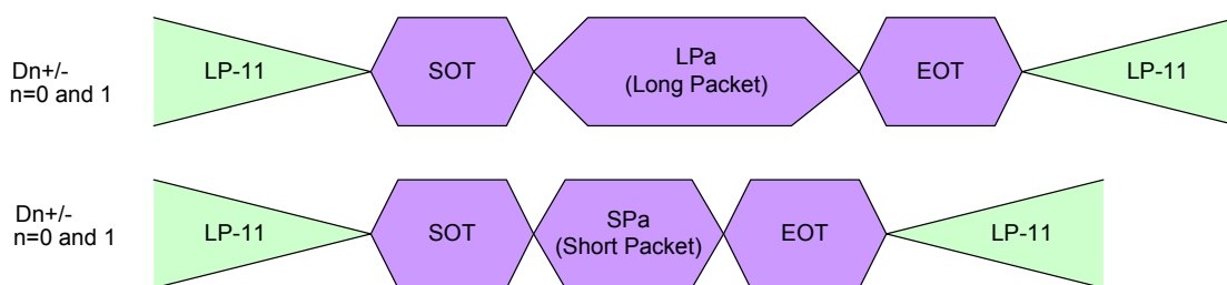
Figure 31 Single Packet in High-Speed Data Transmissions
