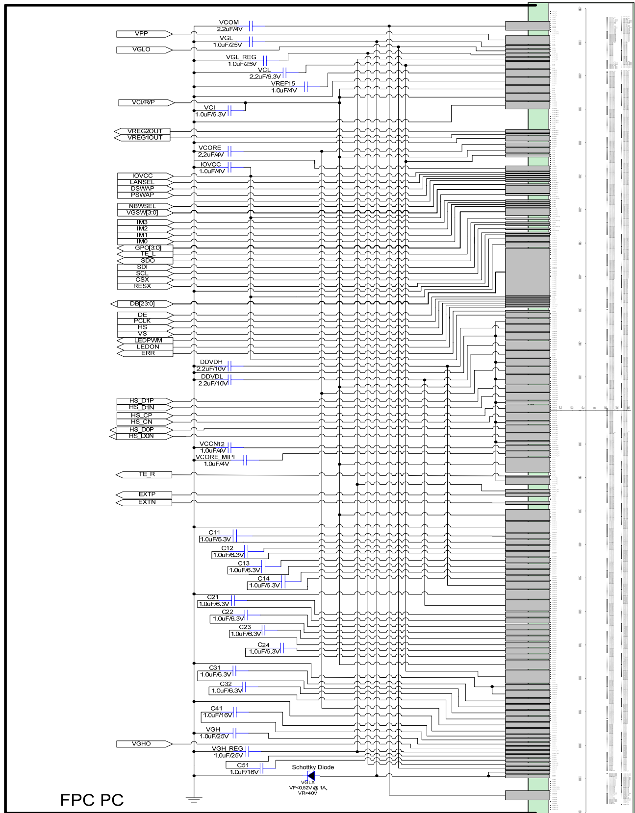
Figure 123 Reference Circuit
