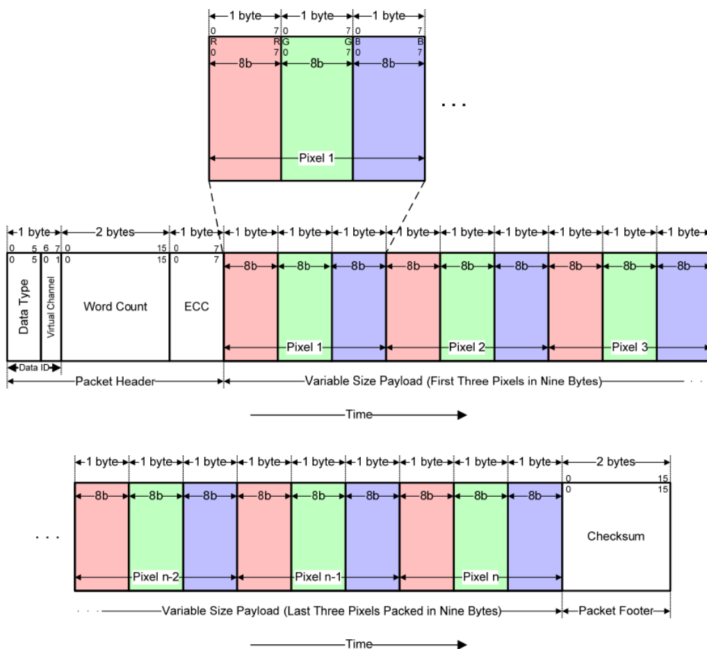
Figure 93 24-bit per Pixel, Data Type = 11 1110 (3Eh)
