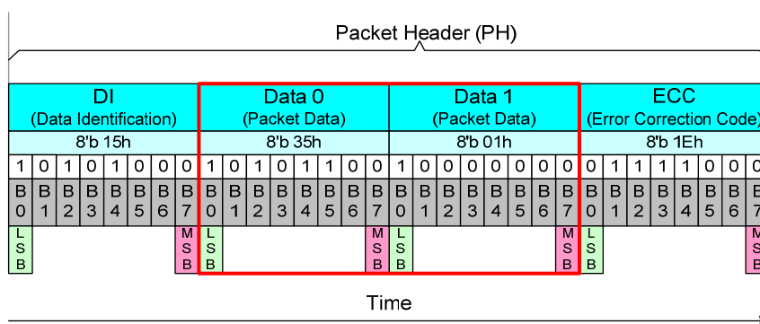
Figure 53 Packet Data (PD) for Short Packet (SPa), 2 Bytes Information
