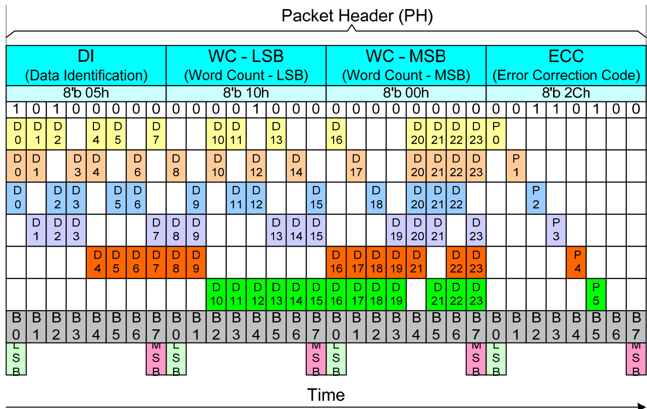
Figure 59 XOR Functionality on the Short Packet (SPa)
