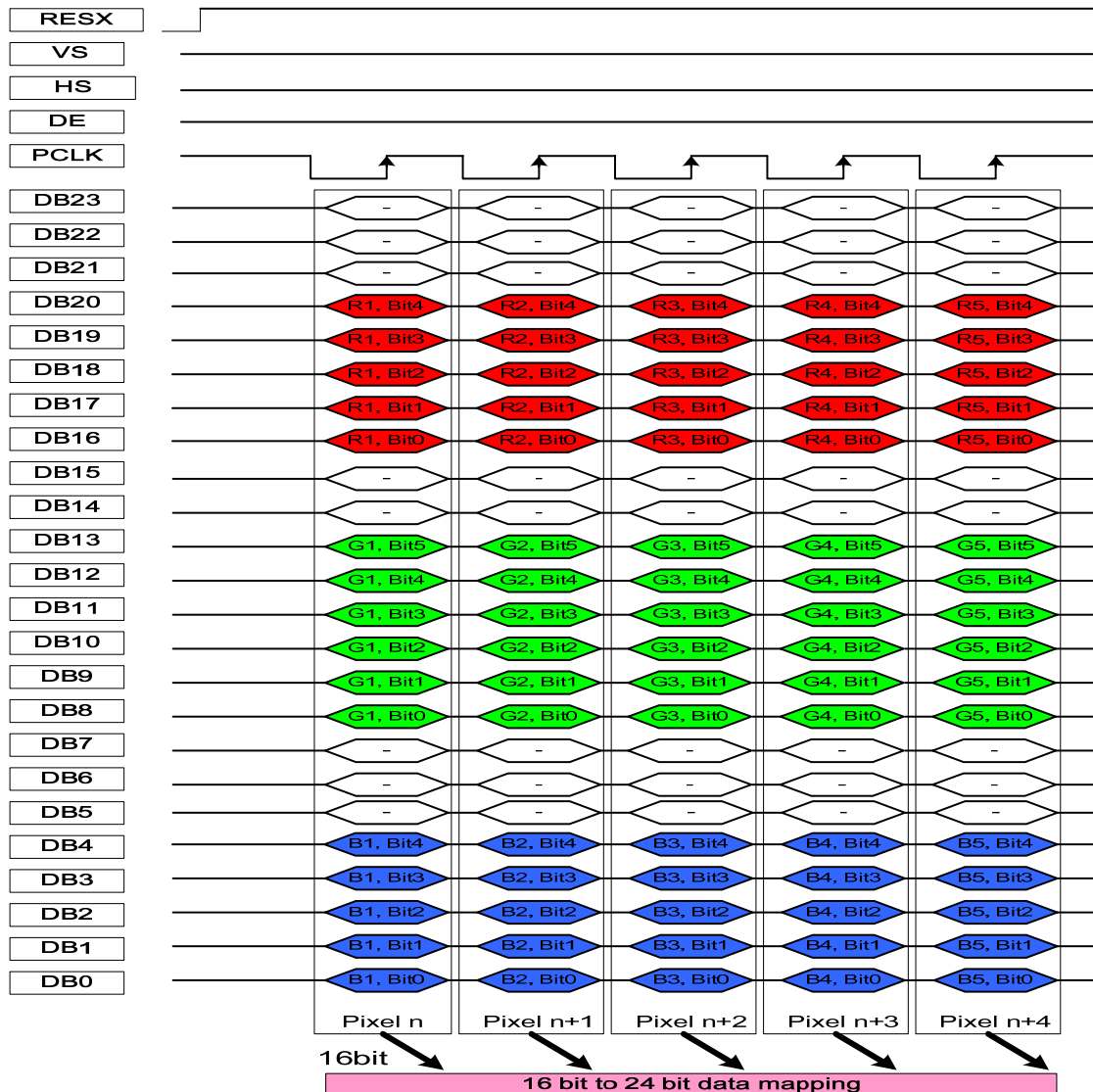
Figure 87 16-bit / pixel 65K colors order on the DPI Interface
