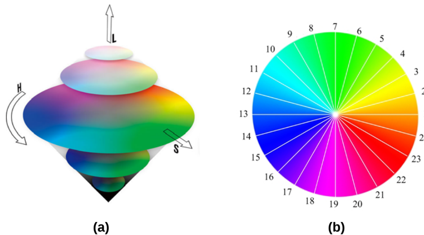
Figure 95 : (a) HSL model, (b) the definition of 24 color-axis.
