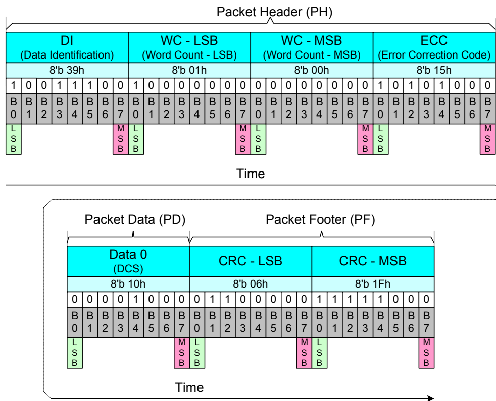
Figure 70 Display Command Set (DCS) Write Long (DCSW-L) with DCS Only - Example
