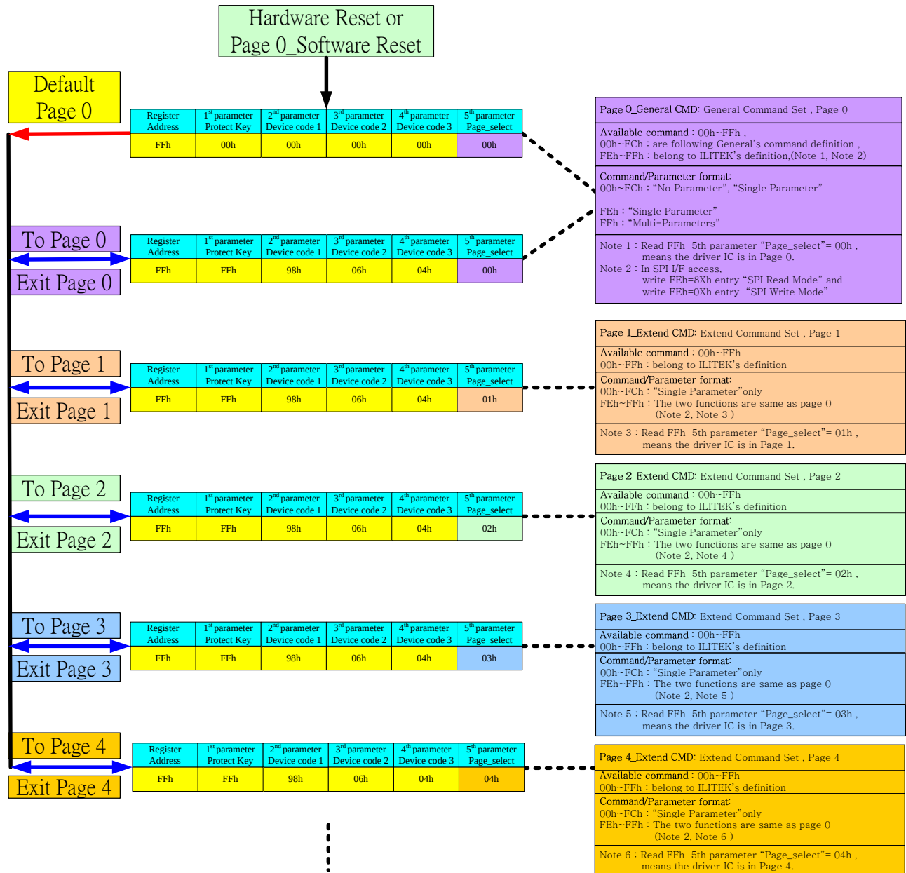
Figure 94 Command Flow
