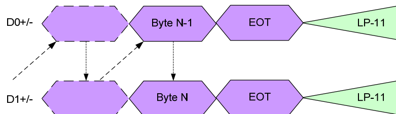
Figure 39 End of Transmission (EoT) in HSDT when Number of Bytes is Equal on Both Data Lanes at the End of the Packet
