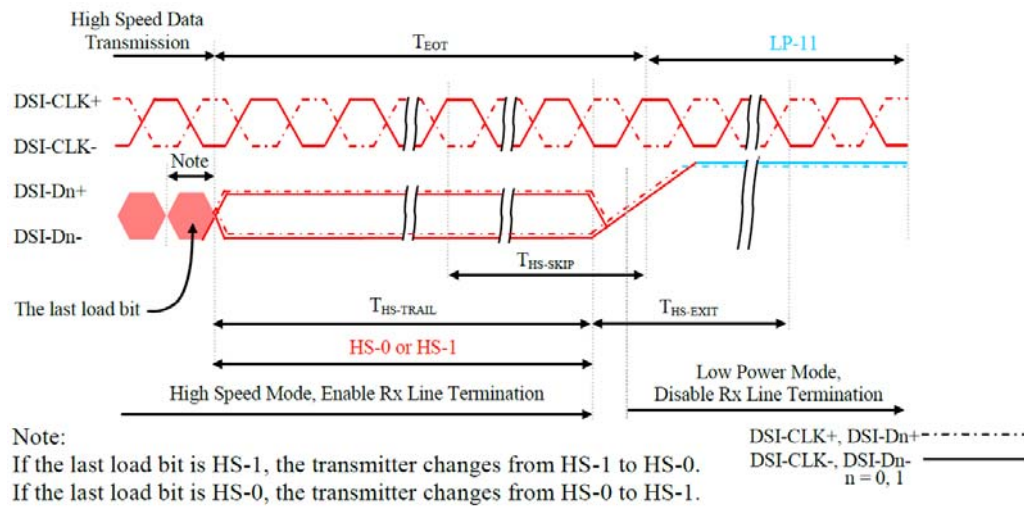
Figure 121 Data Lanes – High Speed Mode to Low Power Mode Timings
