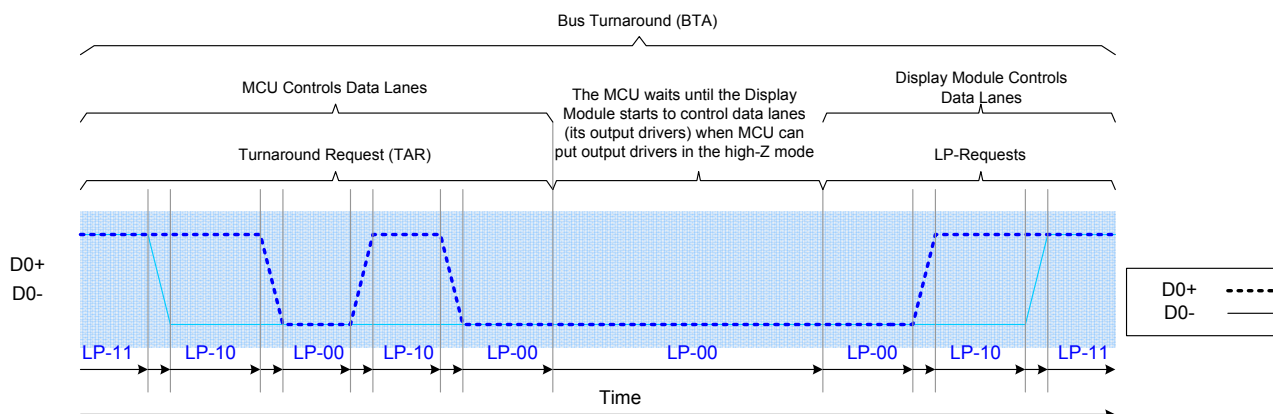
Figure 41 Bus Turnaround Procedure
