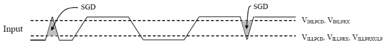
Figure 111 Spike / Glitch Rejection
