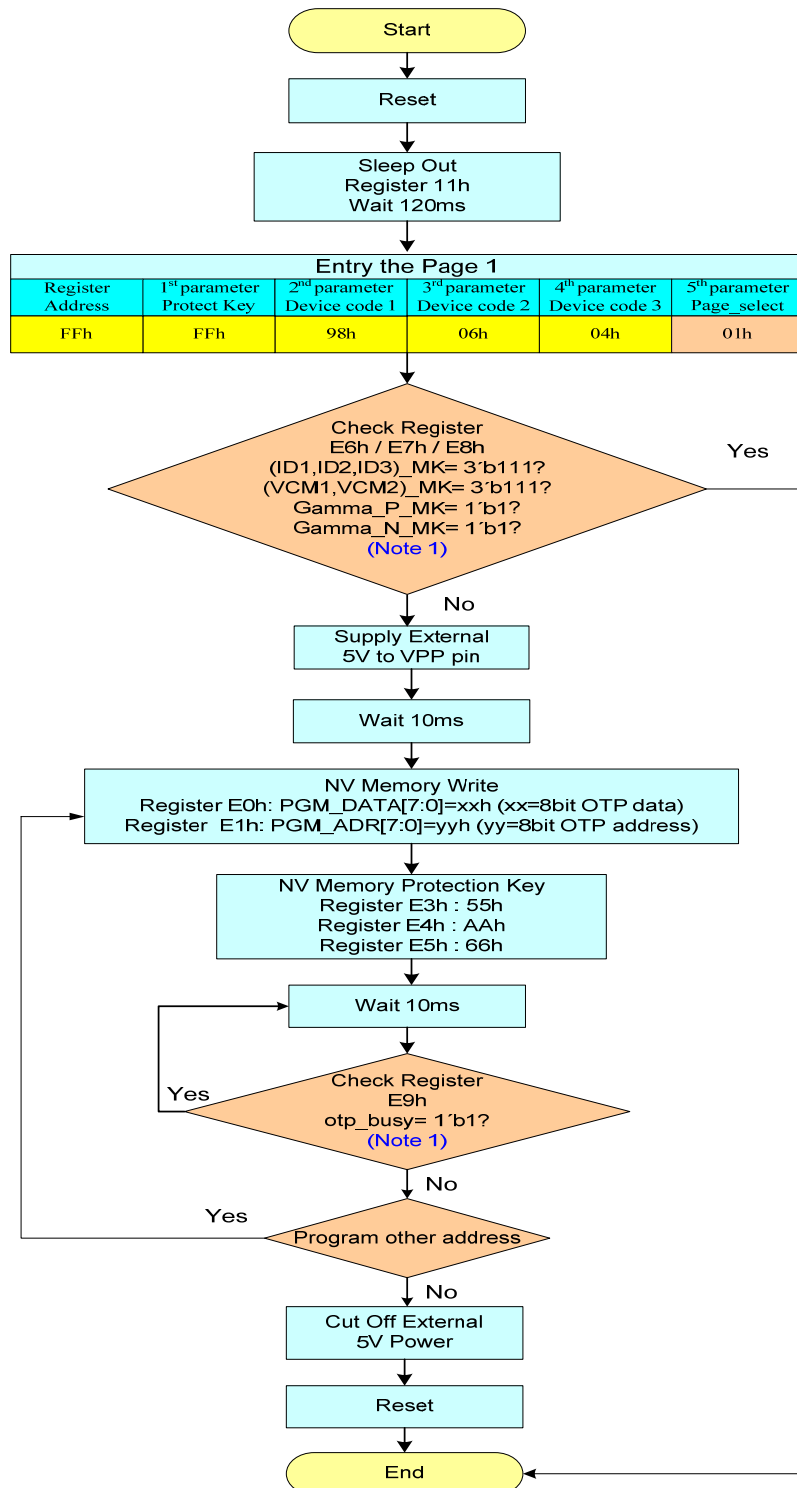
Figure 105 NV Memory Programming Flow
