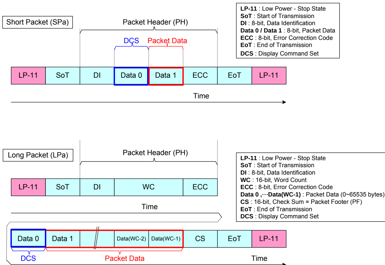
Figure 67 Display Command Set (DCS) on Short Packet (SPa) and Long Packet (LPa)
