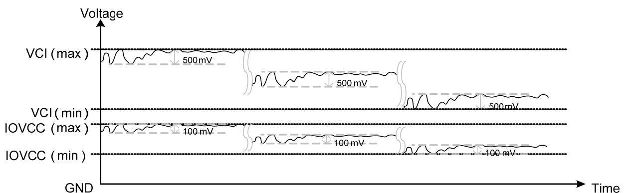
Figure 110 Noise on Power Supply Lines
