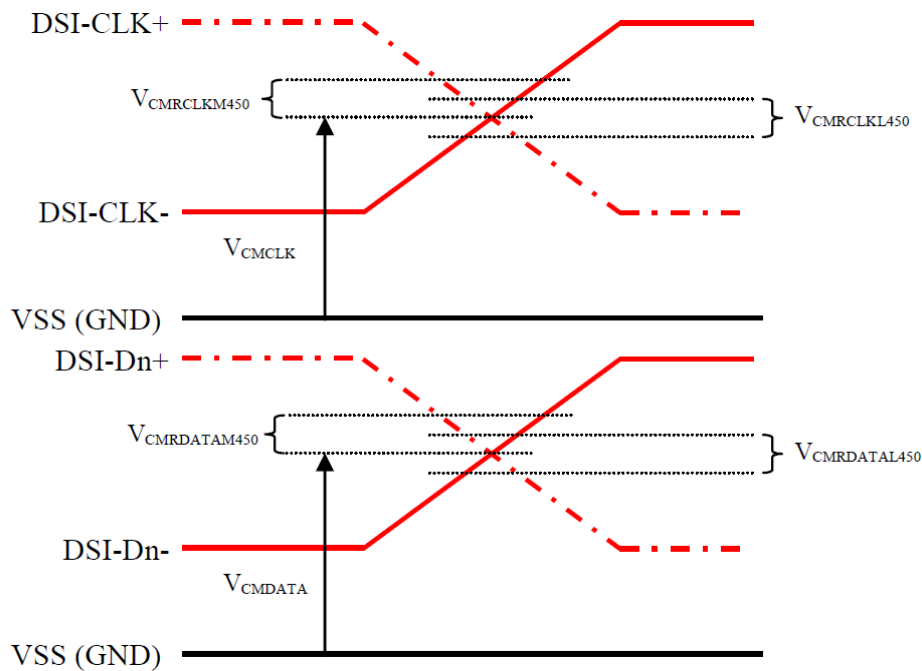
Figure 113 Common Mode Voltage on Clock and Data Channels
