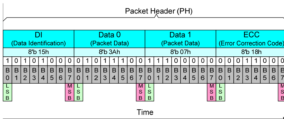
Figure 46 Packet Header (PH) on Short Packet (SPa)
