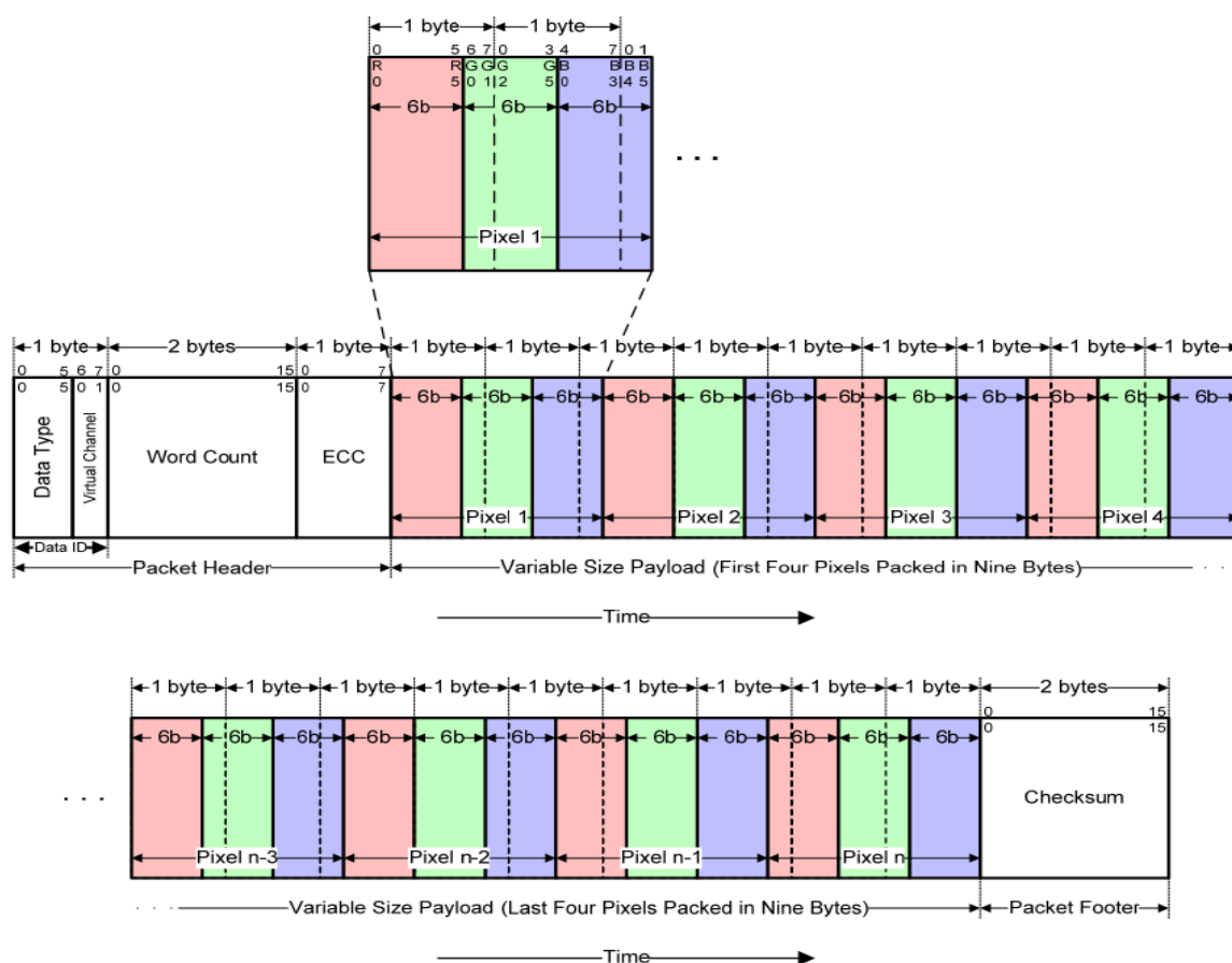
Figure 91 18-bit per Pixel, Data Type = 01 1110 (1Eh)
