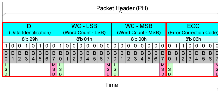
Figure 58 D[23...0] and P[7...0] on the Long Packet (LPa)
