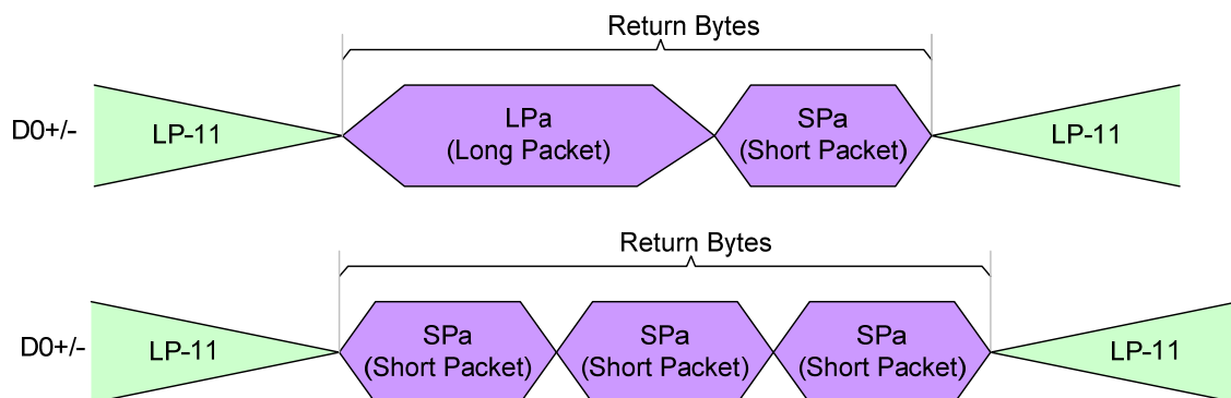
Figure 79 Return Bytes on Several Packets – Not Possible
