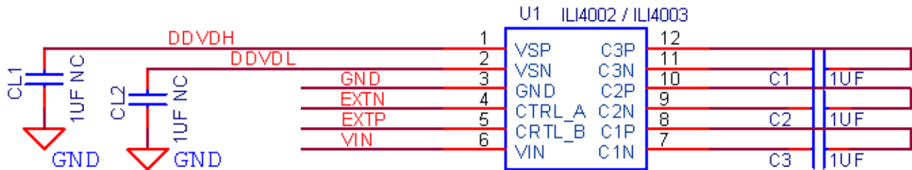
Figure 125 ILI4002/ILI4003 Reference Circuit
