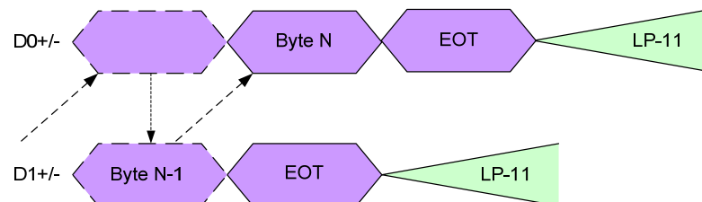
Figure 40 End of Transmission (EoT) in HSDT when Number of Bytes is not Equal on Both Data Lanes at the End of the Packet
