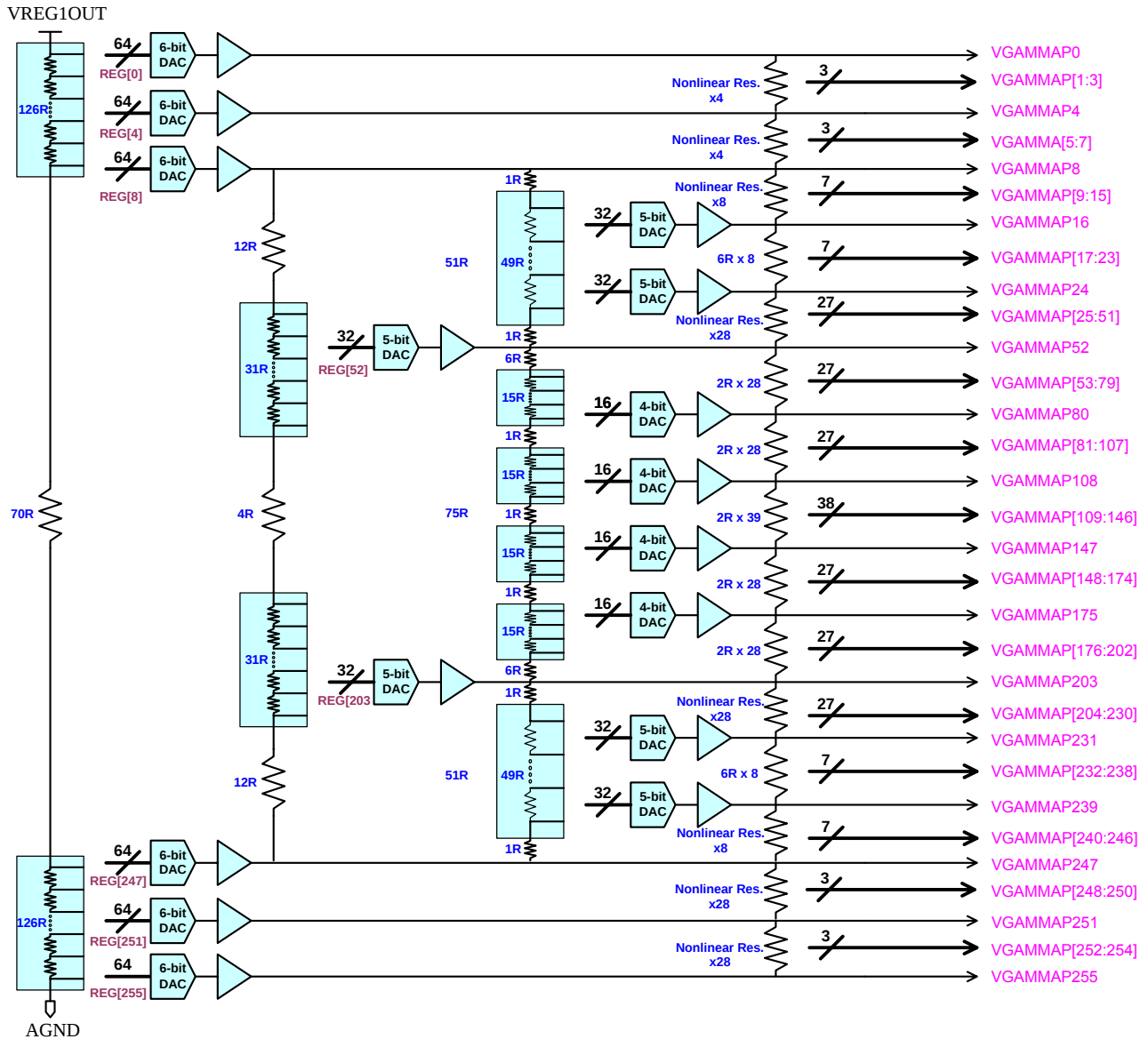
Figure 107 Positive Gamma Control (Page1_A0h~AFh)
