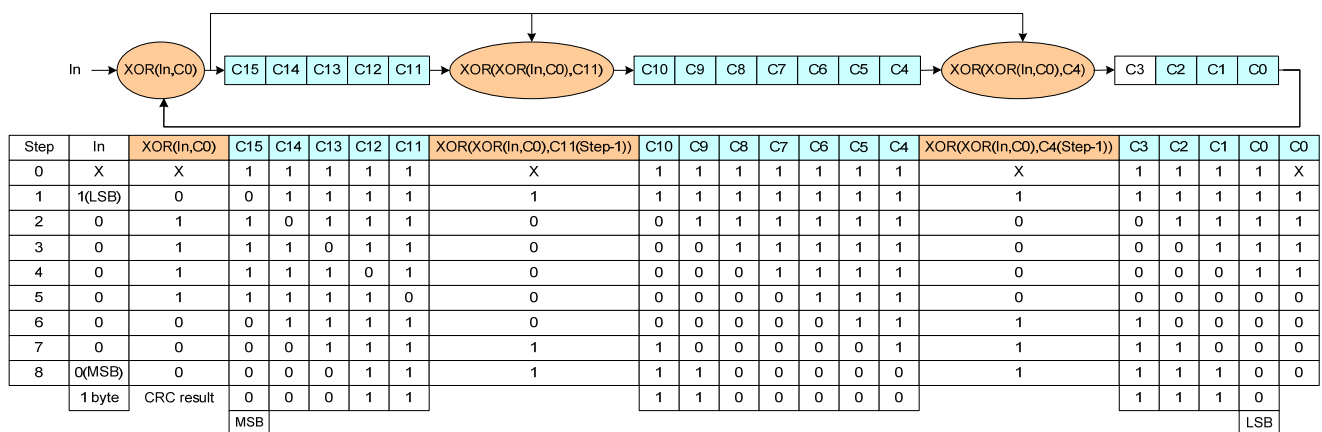
Figure 65 CRC Calculation – Packet Data (PD) is 01h
