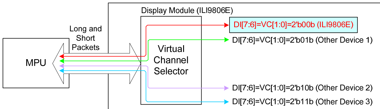
Figure 51 Virtual Channel (VC) Configuration
