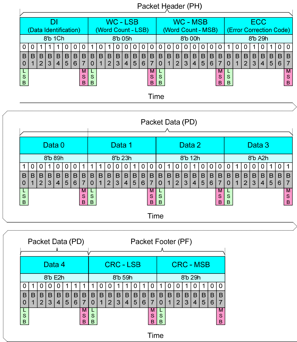
Figure 84 DCS Read Long Response (DCSRR-L) - Example
