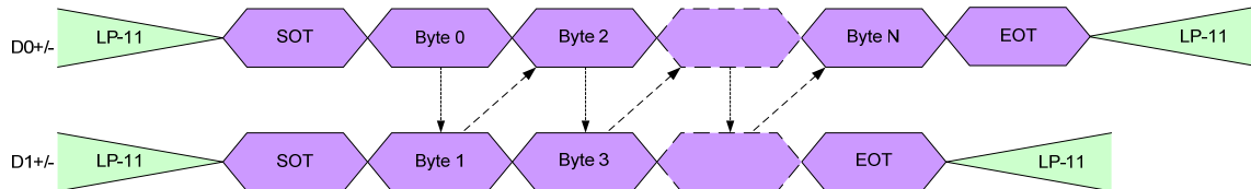
Figure 35 Single Packet in HSDT – Odd Number of Byte
