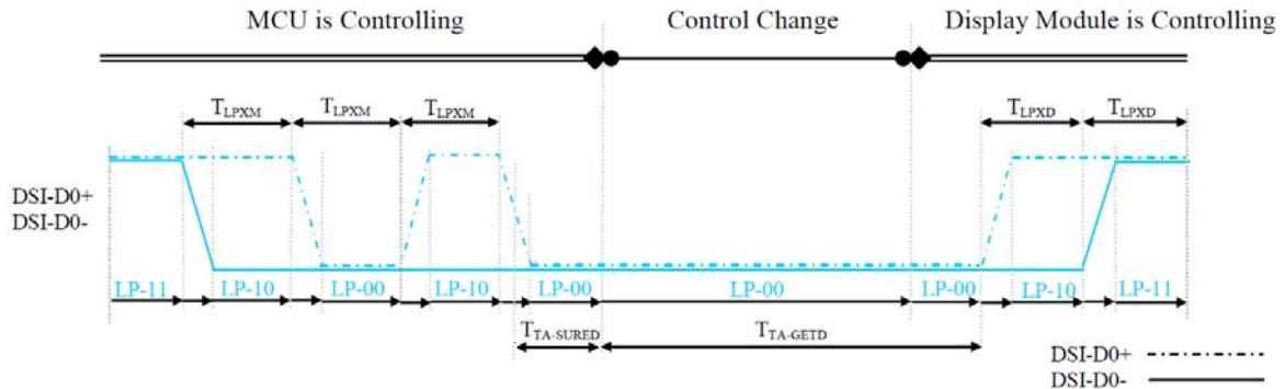
Figure 118 BTA from the MPU to the Display Module
