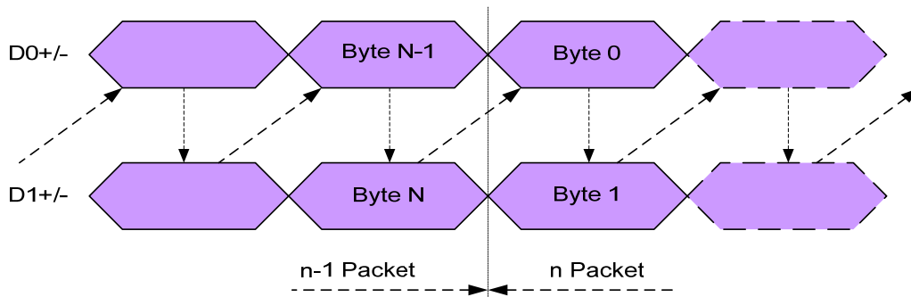
Figure 37 Continue Multiple Packets in HSDT when Number of Bytes is Equal on Both Data Lanes at the End of the Packet
