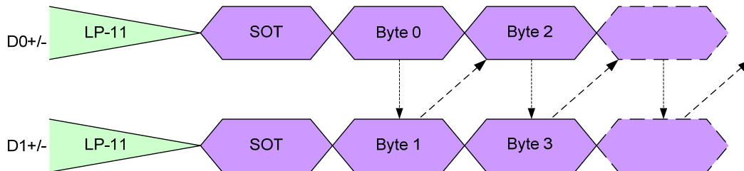
Figure 36 Start of Transmission (SoT) in HSDT for Multiple Packets
