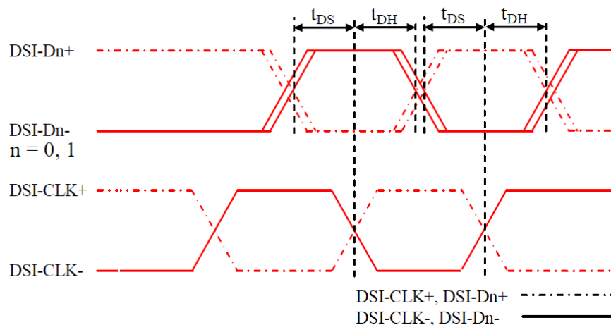
Figure 116 DSI Data to Clock Channel Timings
