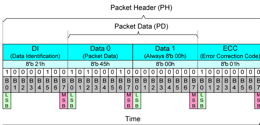
Figure 85 DCS Read Short Response, 1 Byte Returned (DCSRR1-S) - Example
