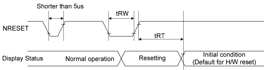
Figure 103 Reset Timing
