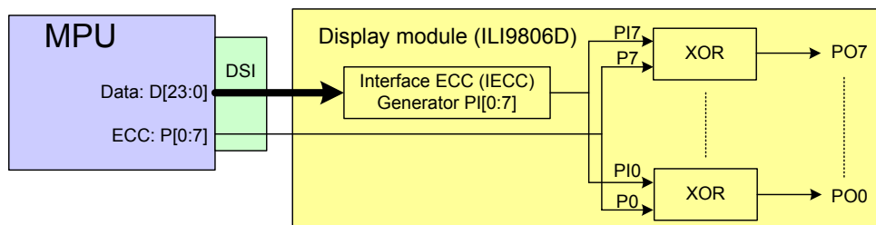
Figure 61 Internal Error Correction Code (IECC) on the Display Module (The Receiver)
