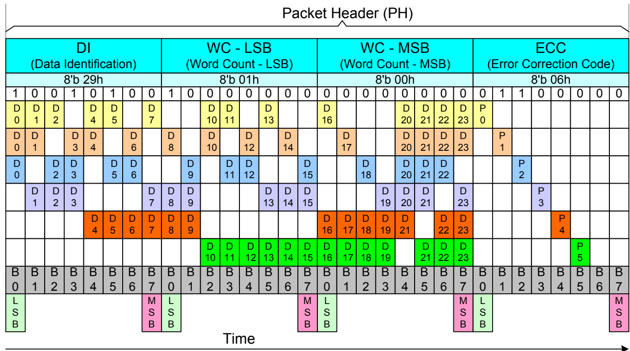
Figure 60 XOR Functionality on the Long Packet (LPa)
