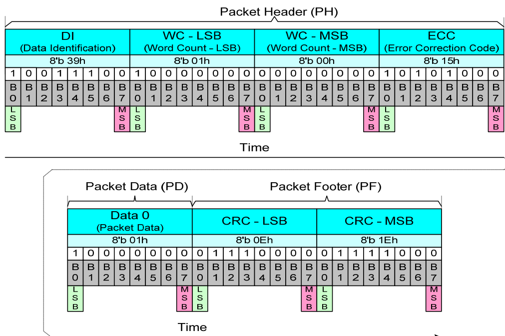
Figure 47 Packet Header (PH) on Long Packet (LPa)
