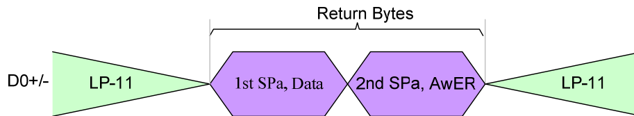
Figure 80 Exception when Return Bytes on Several Packets
