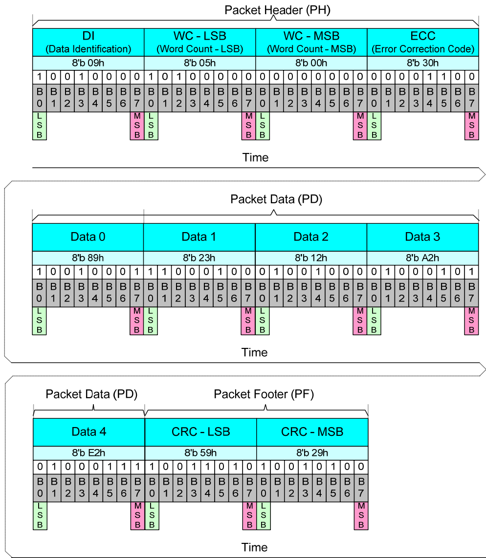
Figure 75 Null Packet, No Data (NP-L) - Example
