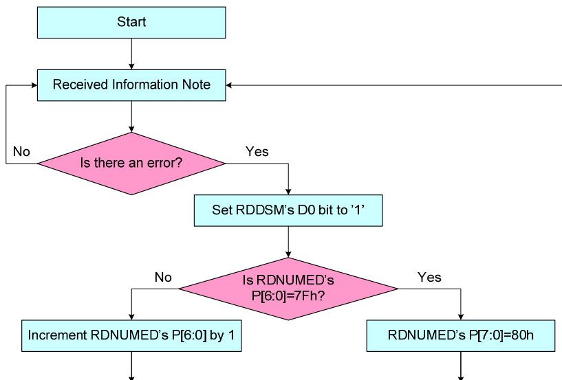
Figure 83 Flow Chart for Errors on DSI Note
