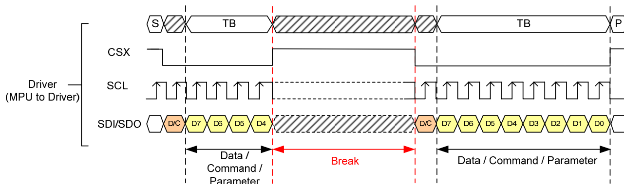
Figure 5 Data Transfer Break and Recovery (SCL rising edge example)
