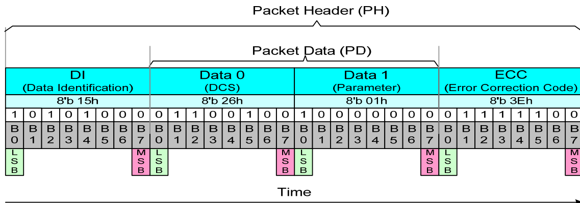
Figure 69 Display Command Set (DCS) Write, 1 Parameter (DCSW1-S) – Example
