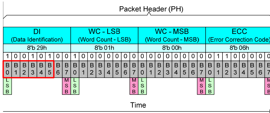
Figure 52 Data Type (DT) on the Packet Header (PH)
